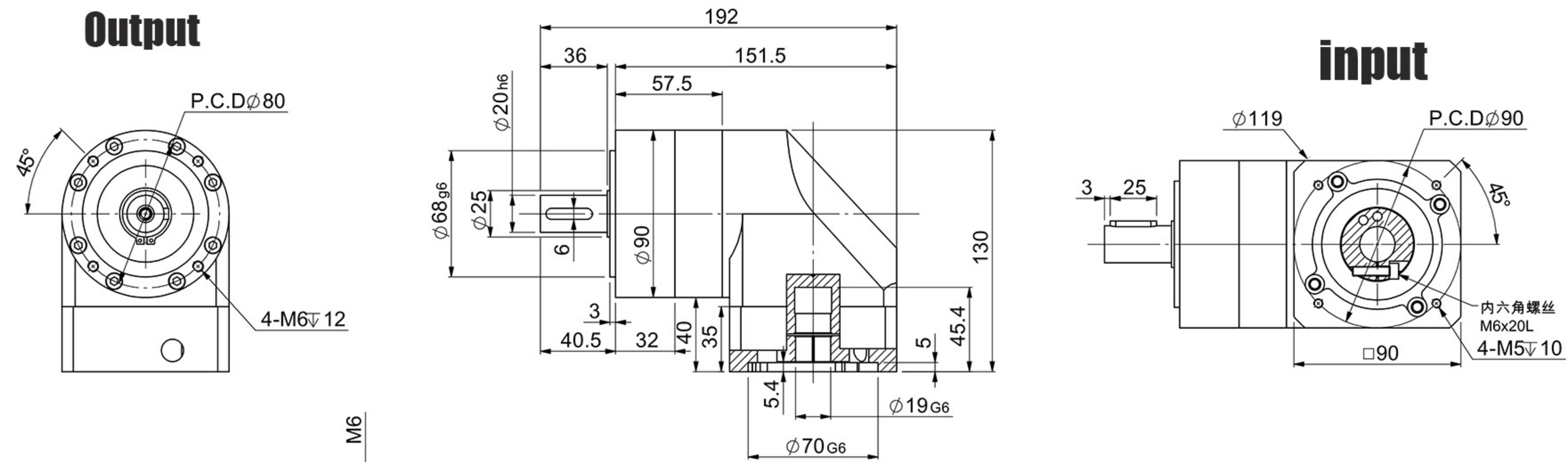
Level 1(Ratio)Drawing: 3:1; 4:1; 5:1; 7:1; 10:1
